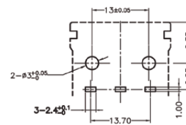
PCB LAYOUT THICKNESS: 0.8~1.6t
