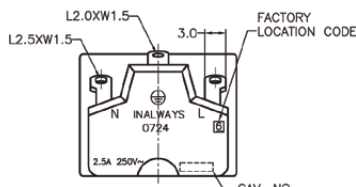
VIEW "B"
